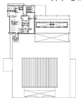
3F PLAN
